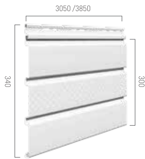
SV(P) 07 (Infratop) Panel with perforation
